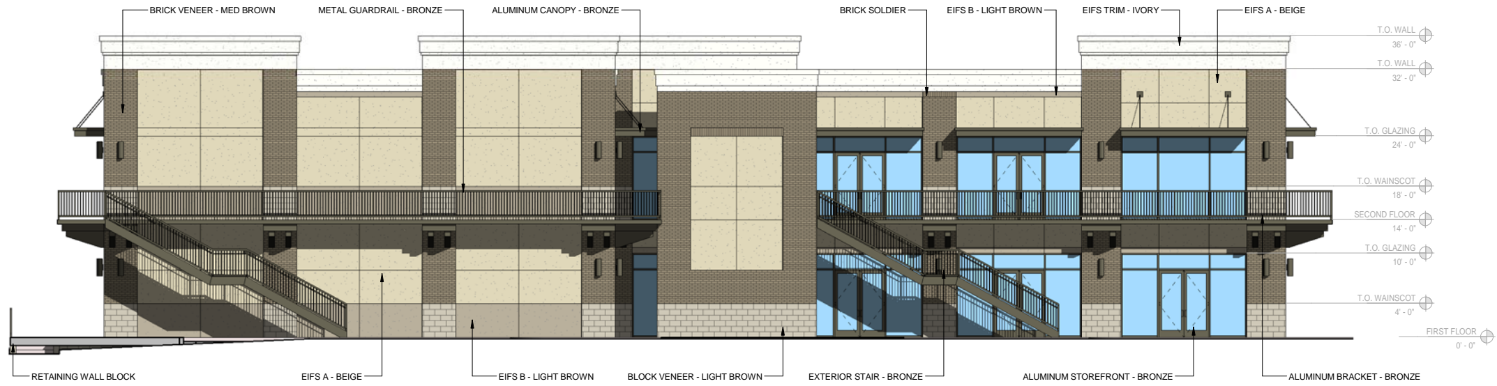
② SCHEMATIC WEST ELEVATION 1/8" = 1'-0"
