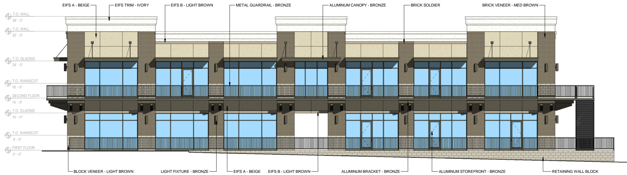
② CHAMBLEE DUNWOODY RD ELEVATION 1/8" = 1'-0"
